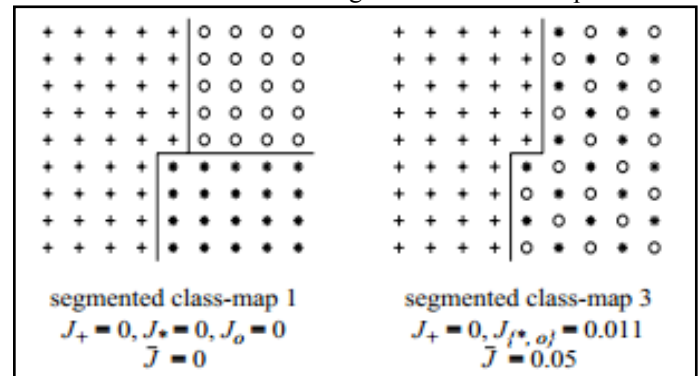
Fig. 3: Segmented Class-maps and their Corresponding J Values
