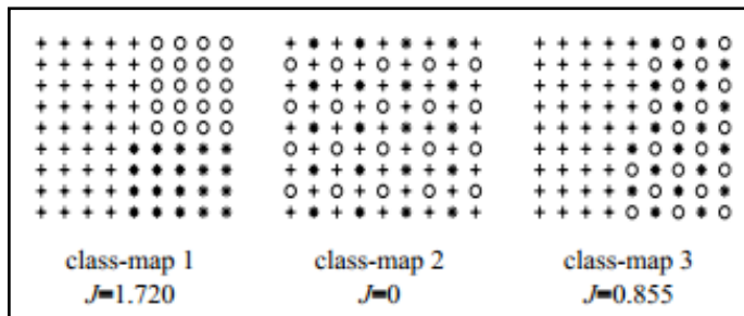
Fig. 2: An Example of Different Class-maps and their Corresponding J value. '+', 'o', and '*' Indicate Three Classes of data Points.
