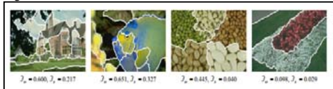
Fig. 7: Example Segmentation Results on Images from Photo CDs 2,500 Images are automatically Processed Without any Parameter Tuning on Individual Images. 1 Scale, Size 192x128, \bar{J}_o is \bar{J} Calculated for the Original Image and \bar{J}_s is for the Segmented One.
