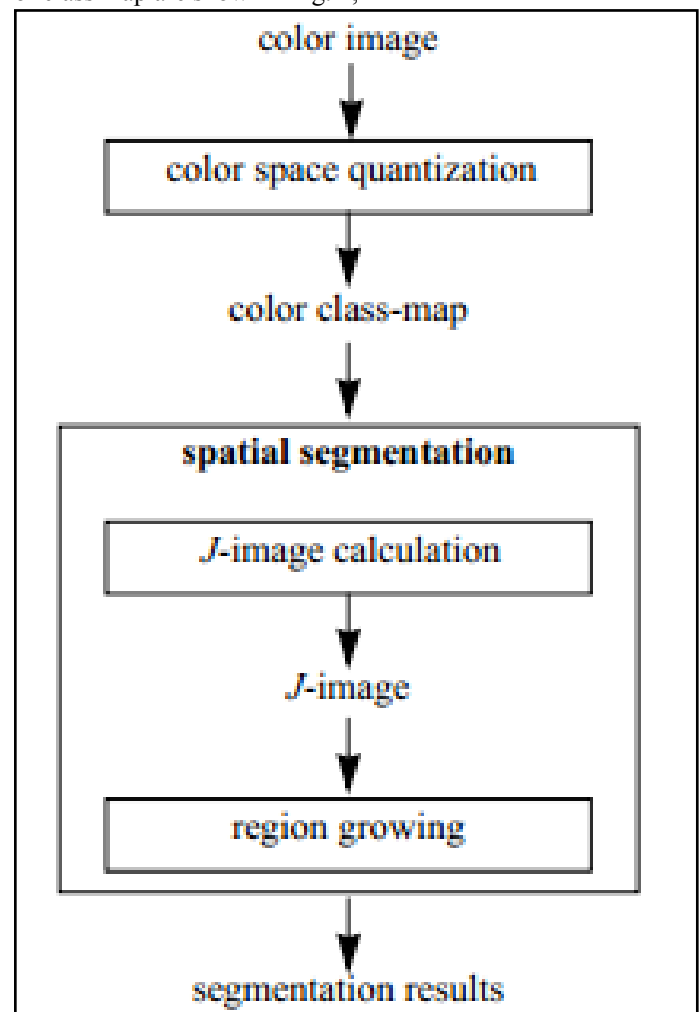
Fig. 1: Schematic of the JSEG Algorithm
