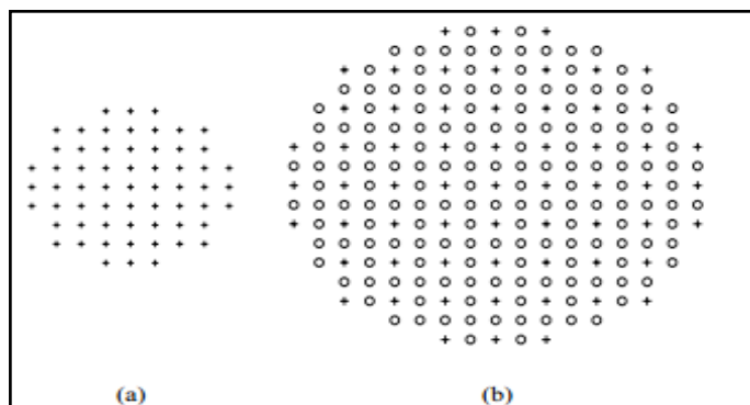
Fig. 4: (a). The Basic Window for Calculating Local J Values. (b). Illustration of Downsampling for the Window at Scale 2. Only '+' Points are Used for Calculating Local J Values, Which forms the Same Basic Window as in (a).
